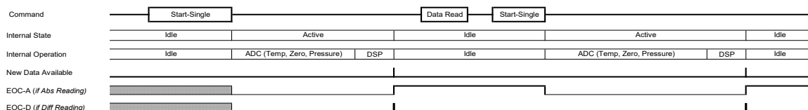
Figure 2 - AUAV Communication Model
