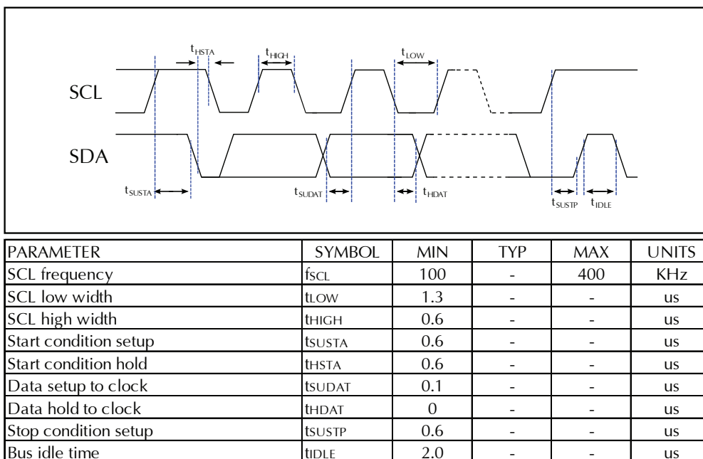
Figure 5 - I2C Timing Diagram
