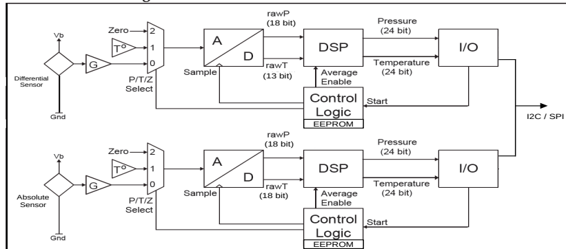
Figure 1 - AUAV Block Diagram
