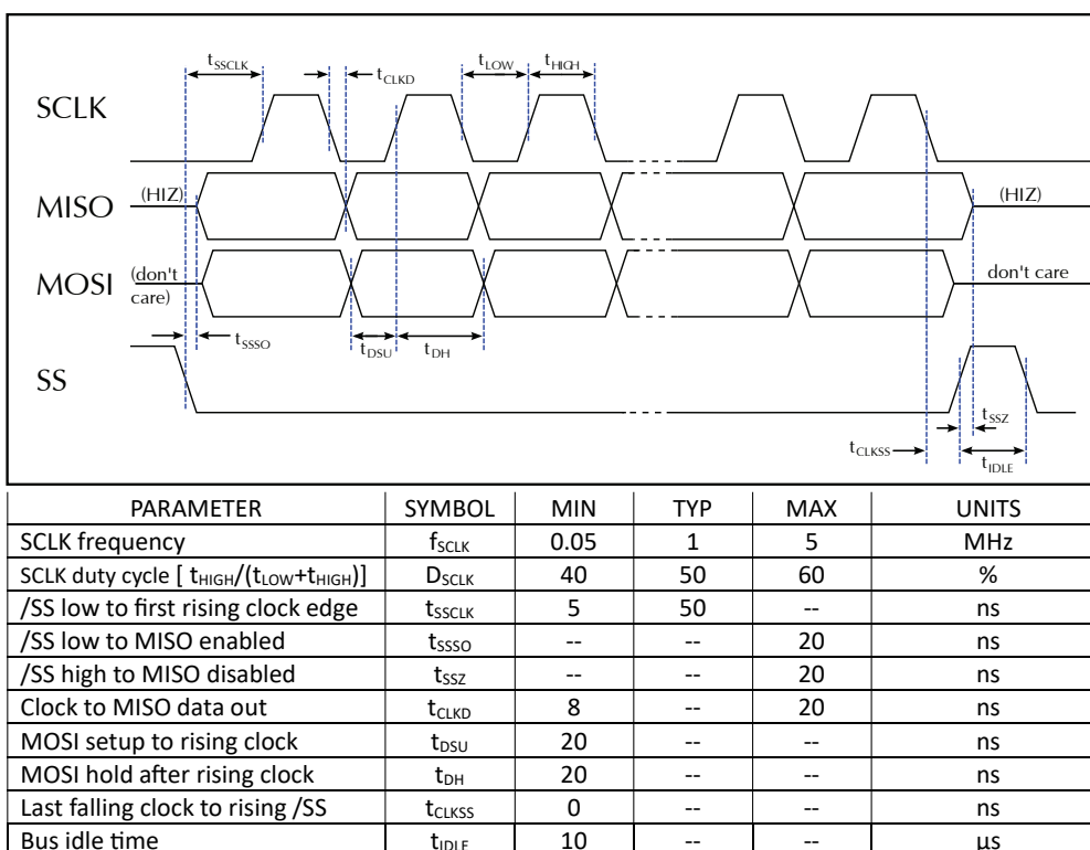
Figure 6 - SPI Timing Diagram
