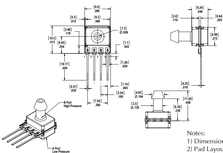
SIP H-Lead AN: Barbed Top Port Gage
