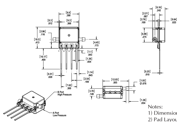
SIP H-Lead DR: Barbed Opposite Side Port Differential
